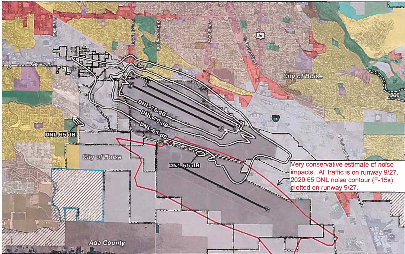
Figure 5-3 2020 Noise Exposure Map on Future Land Use
