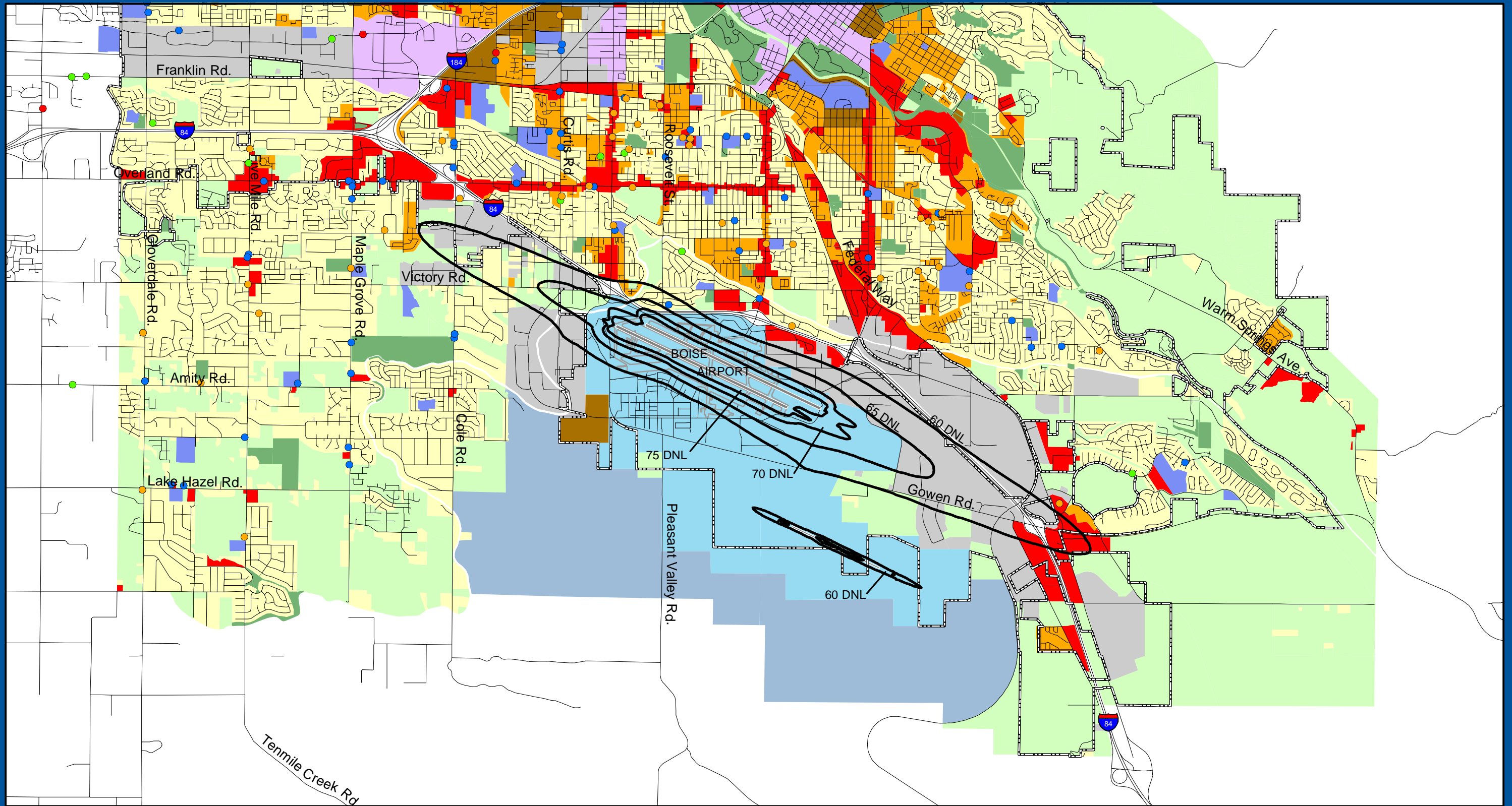
FIGURE 5-1 BOISE AIRPORT 14 CFR PART 150 UPDATE 2004 NOISE EXPOSURE MAP ON EXISTING LAND USE
