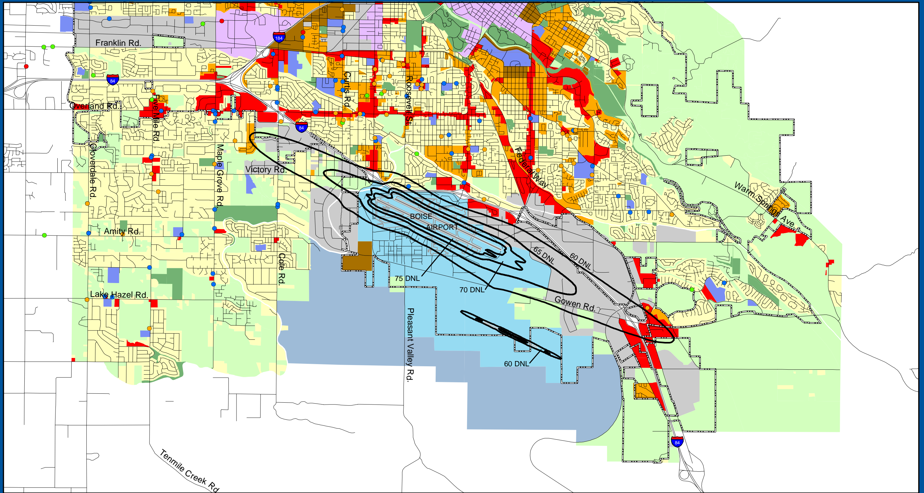
FIGURE 5-2 BOISE AIRPORT 14 CFR PART 150 UPDATE 2009 NOISE EXPOSURE MAP ON EXISTING LAND USE
