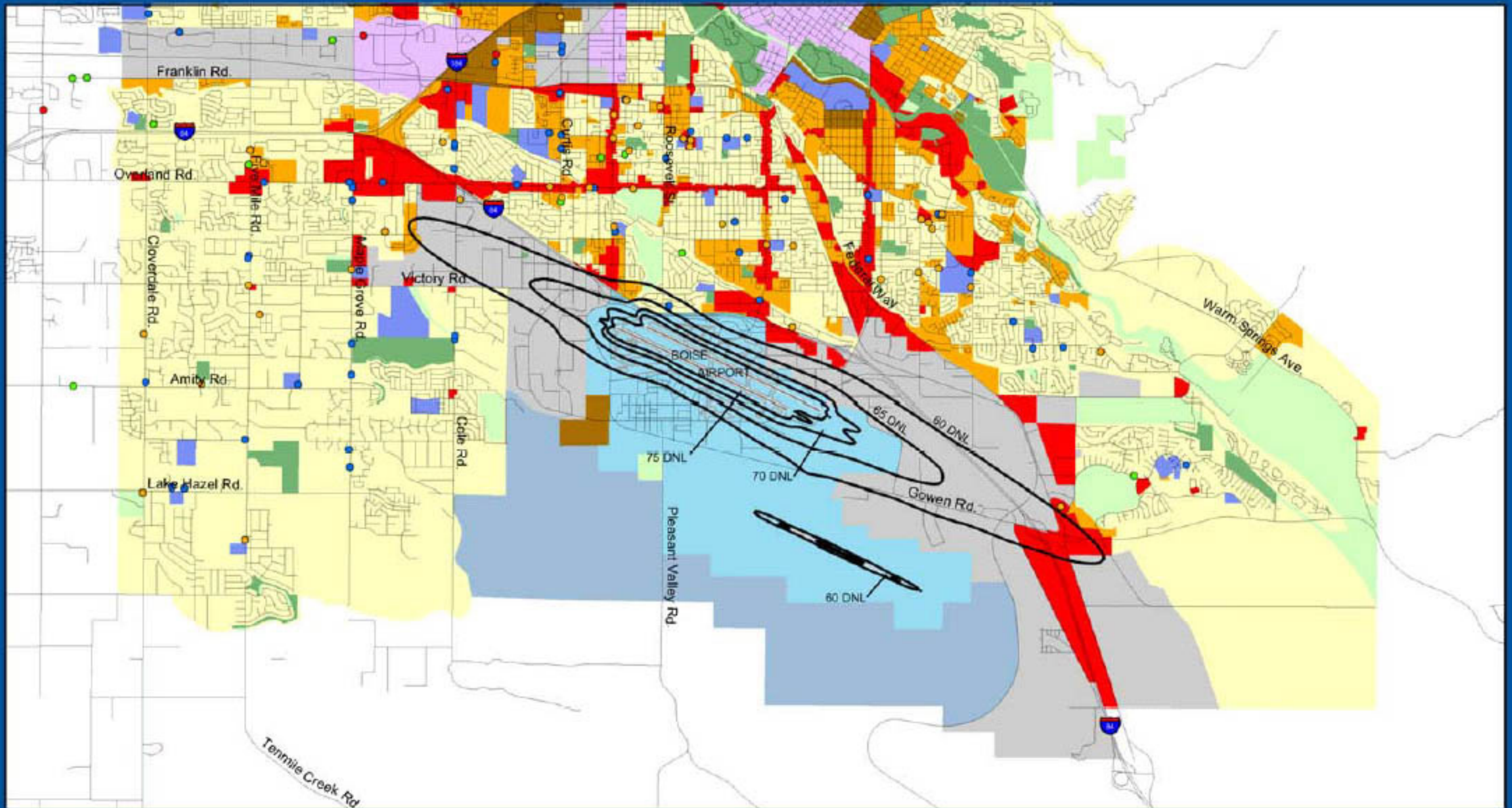
FIGURE 7-3 BOISE AIRPORT 14 CFR PART 150 UPDATE DRAFT 2008 NOISE EXPOSURE MAP ON FUTURE LAND USE
